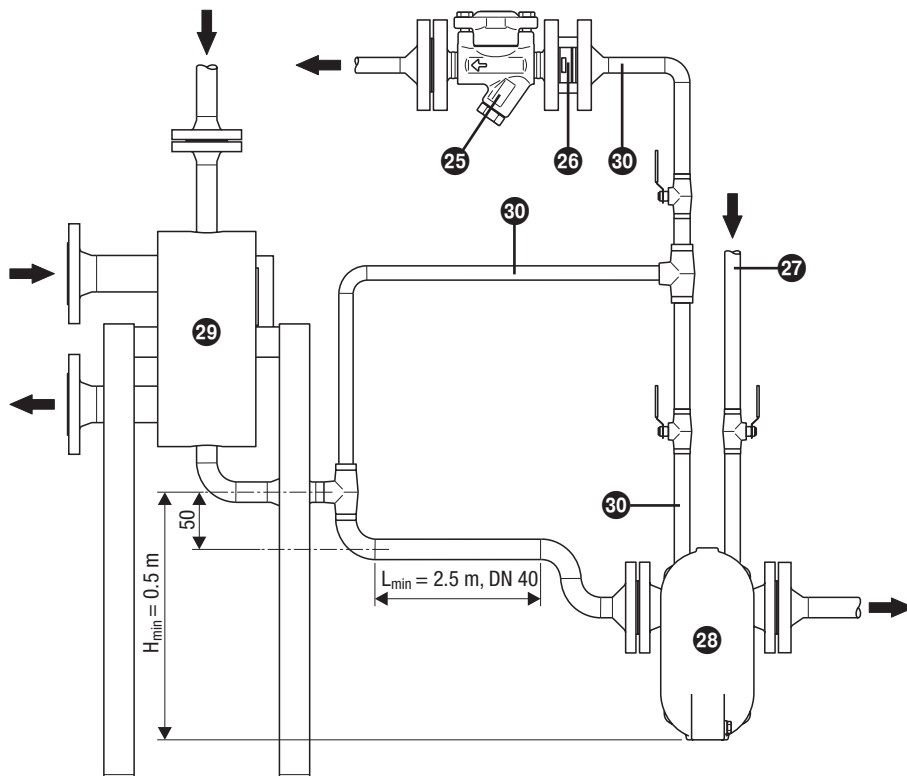
Connection of UNA 25-PK to a heat exchanger
